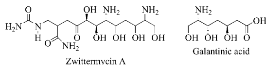
Figure 1. Natural long-chain aminopolyols.
